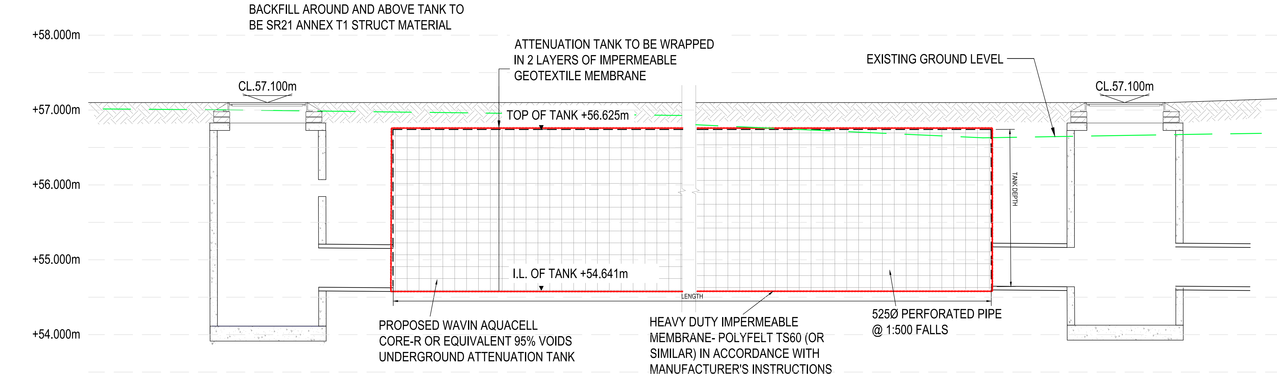
SECTION 1 - UNDERGROUND ATTENUATION TANK SECTION SCALE 1:25
