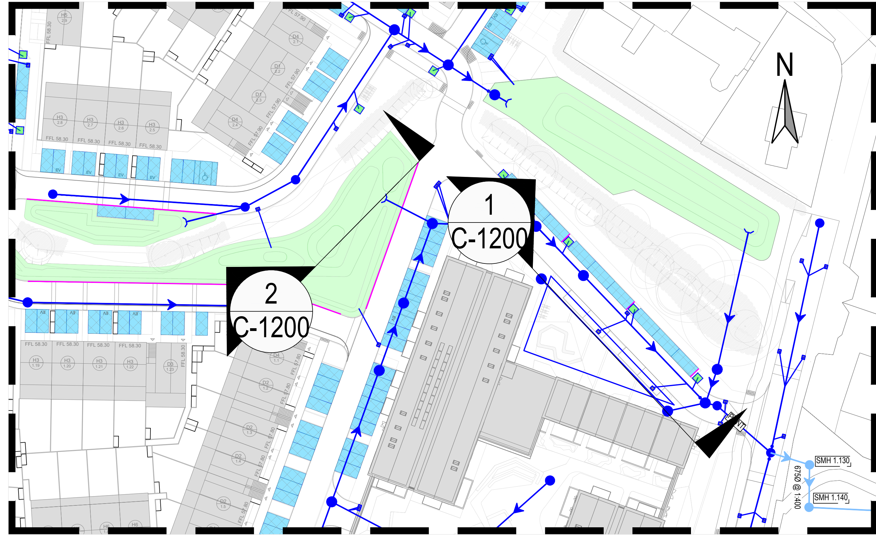
ATTENUATION SECTION PLAN SCALE 1:500
